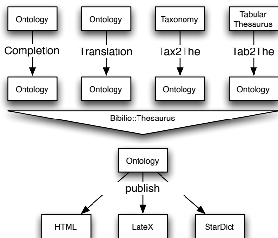
Figure 1: Ontology Algebra
